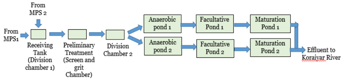
Figure 2.4: STP Components
