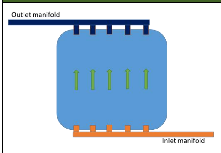
Figure 5.8: Multiple inlet and outlet structures
