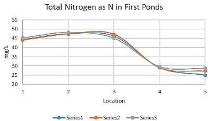
Figure 2.16: Graph of Nitrogen in Maturation Ponds
