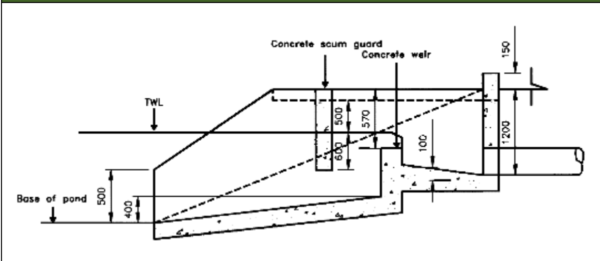
Figure 5.7: Pond outlet structure
