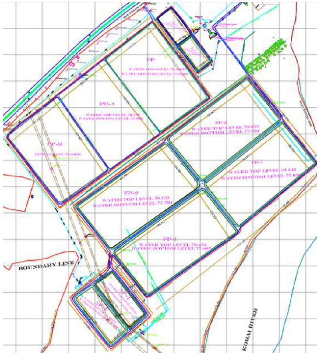
Figure 2.3: STP layout
