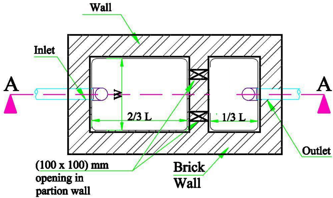
Figure 1: Septic Tank plan
