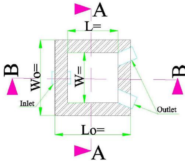
Figure 3: Register for Twin pit
